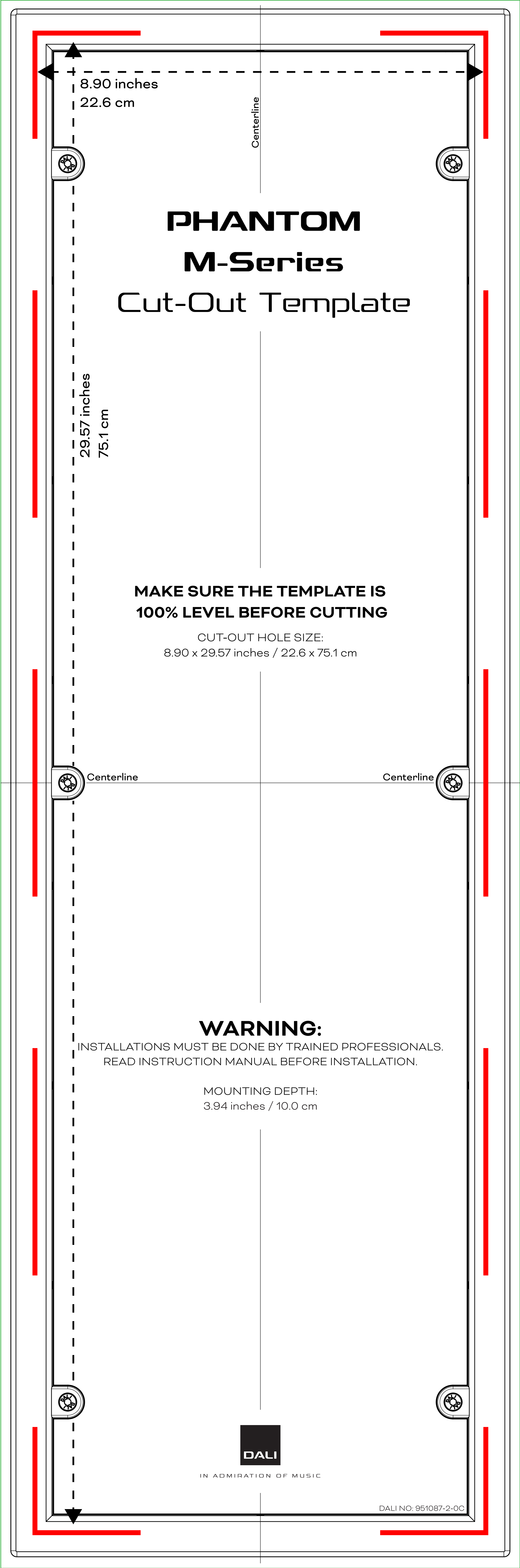
951087-2-0 CUT-OUT TEMPLATE PHANTOM M-250 AND M-375
